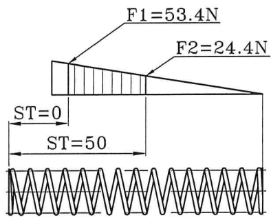
Spring force
